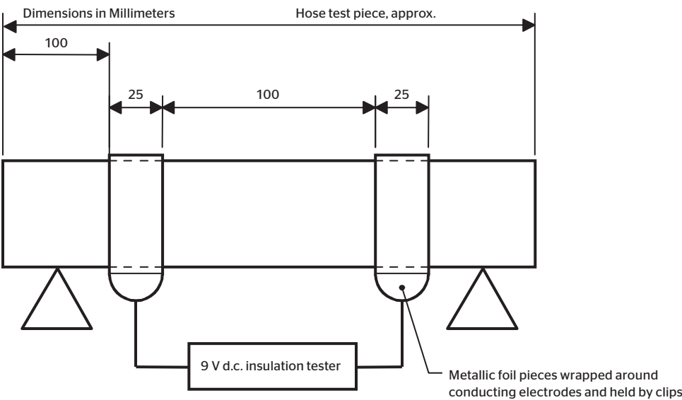
Figure 6-1 – Electrodes and contacts for testing hose
